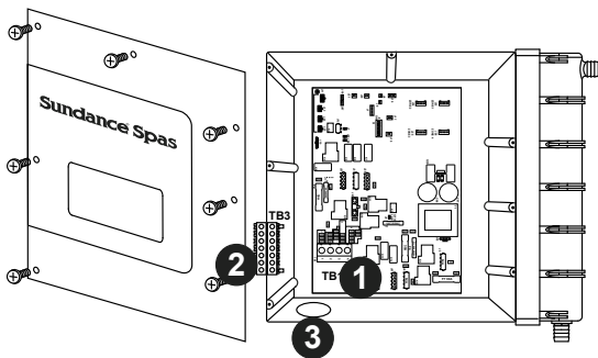
Figure C Control Box
