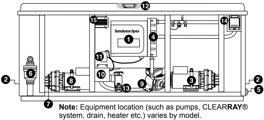
Figure B (Equipment Area for All Models Except Maxxus/Aspen)
