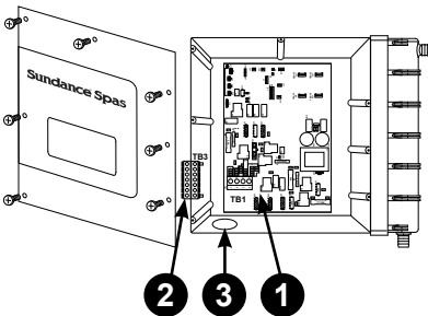
Figure C Control Box 60 Hz
