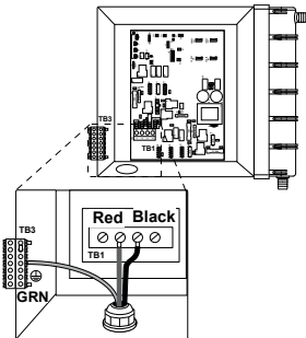
Figure D Terminal Block 240V Wire Connection
