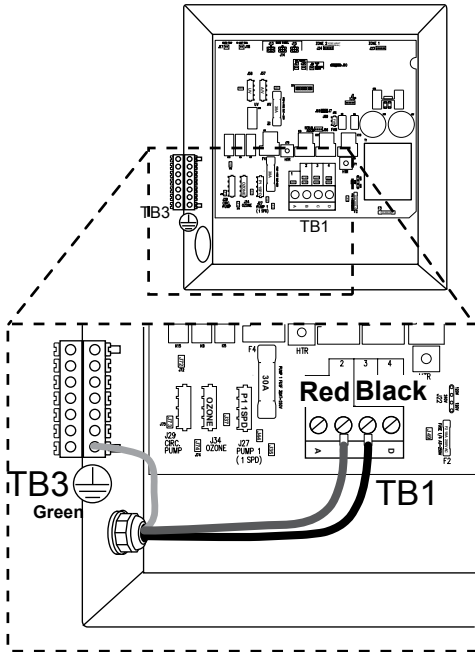
Figure C Connections
