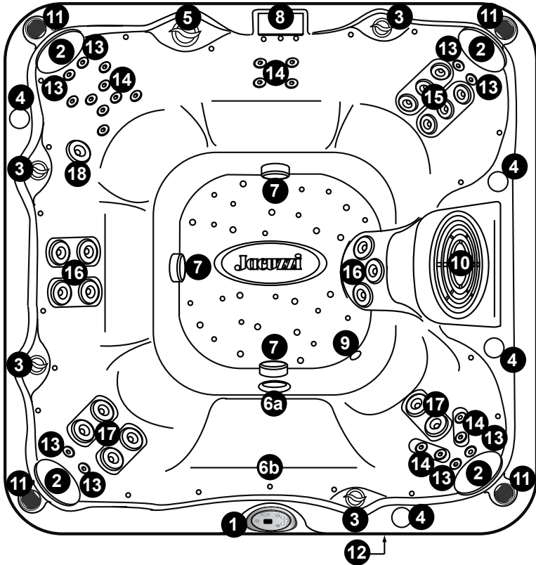
J-280 model illustrated - Jet locations and features vary by model.
