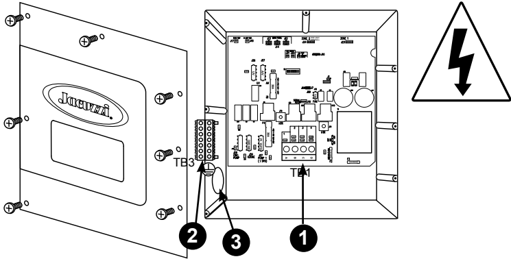
Figure B Control Box
