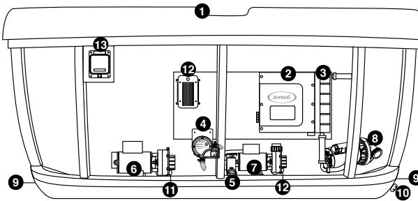
Figure 6.0c Equipment Area
