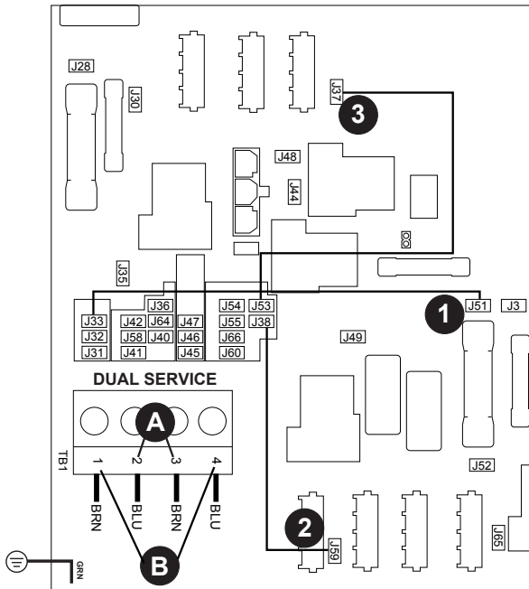
PARTIAL VIEW OF THE CIRCUIT BOARD
