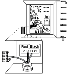
Figure 6.0e Terminal Connections (North American 60Hz 240 VAC Connection Shown)
