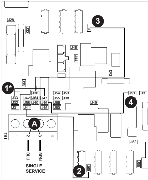
PARTIAL VIEW OF THE CIRCUIT BOARD
