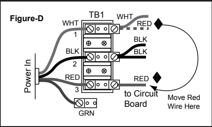
North American Convertible Models: 240 VAC, 4-Wire Connection 60 Hz
