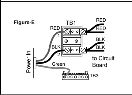
North American 240V Models: 240 VAC, 3-Wire Connection 60 Hz
