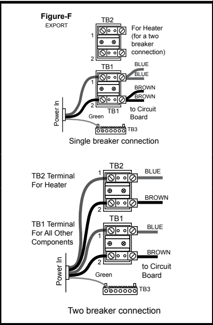
All Export Models: 230 VAC, 3-Wire Connection 50 Hz
