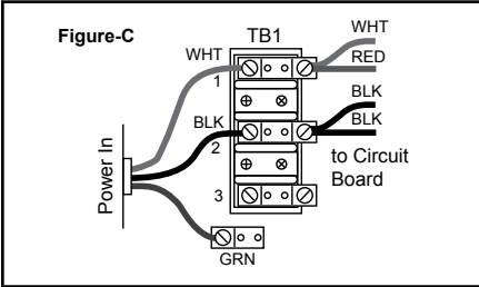
North American Convertible Models: 120 VAC, 3-Wire Connection 60 Hz
